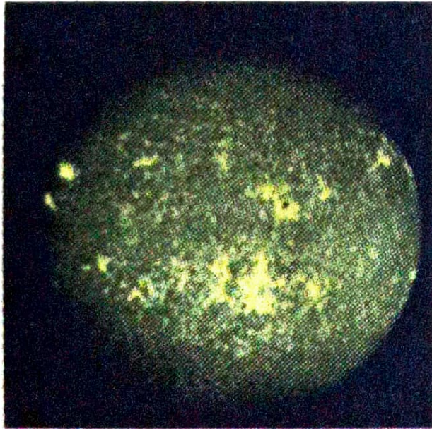
Chromosphere, Sunspots, Plages, Quiet Sun, filaments
